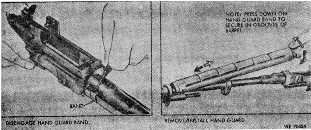
Figure 2-4. Remove/install hand guard.
